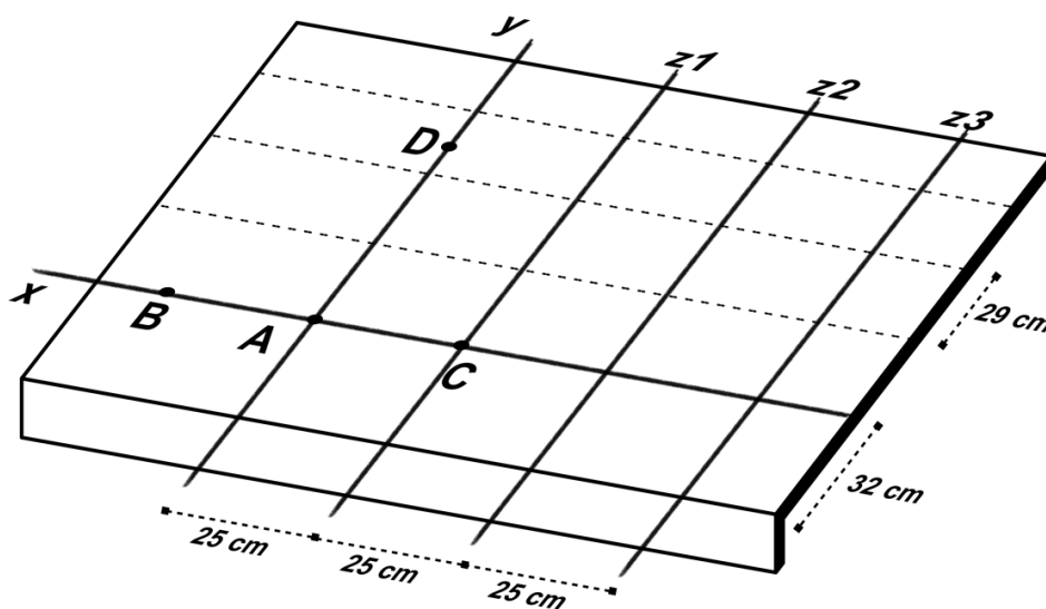
Fig. 26 - Tracing of the pitch [cm] - version 2
