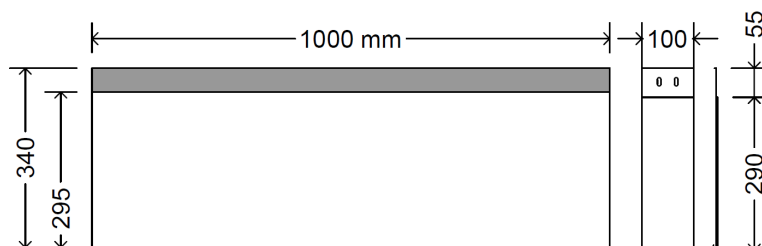
Fig. 1 - Ultimetel HD shingle dimensions
