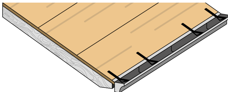
Fig. 2 - Gutter installation
