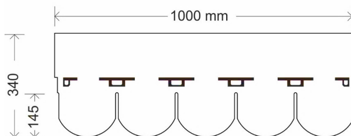
Fig. 1 - Traditional shingle dimensions
