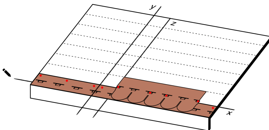
Fig. 7 - Shingles installation
