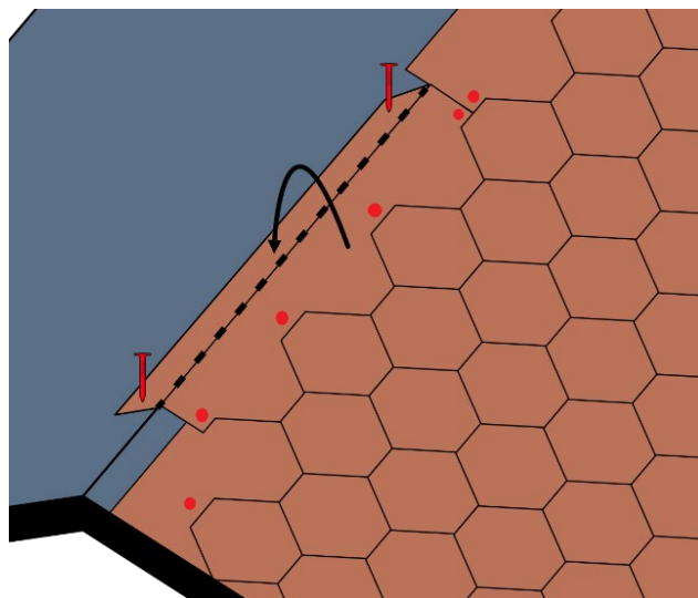
Fig. 9 - Shingles installation at the ridge
