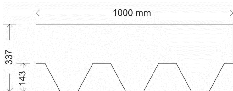
Fig. 1 - Mosaik shingle dimensions
