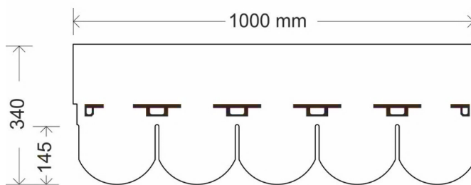
Fig. 1 - Traditional shingle dimensions
