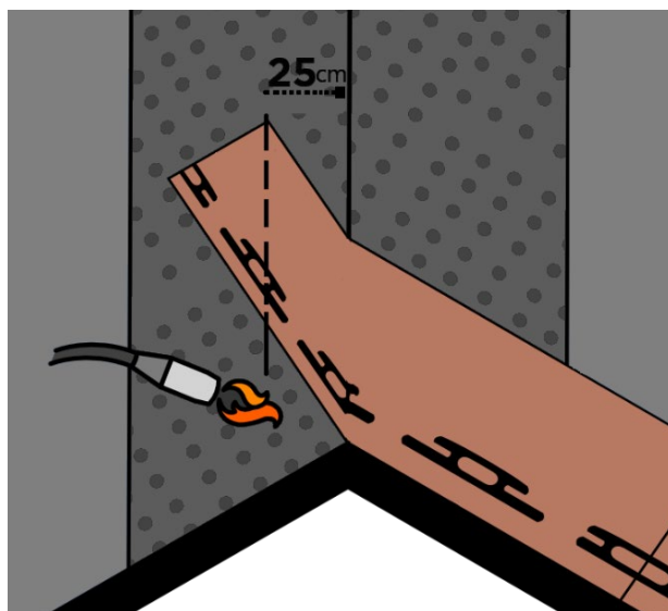
Fig. 20 – Shingles installation by torch at the valley
