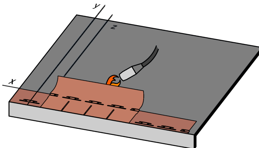
Fig. 17 - First row shingles installation by torch
