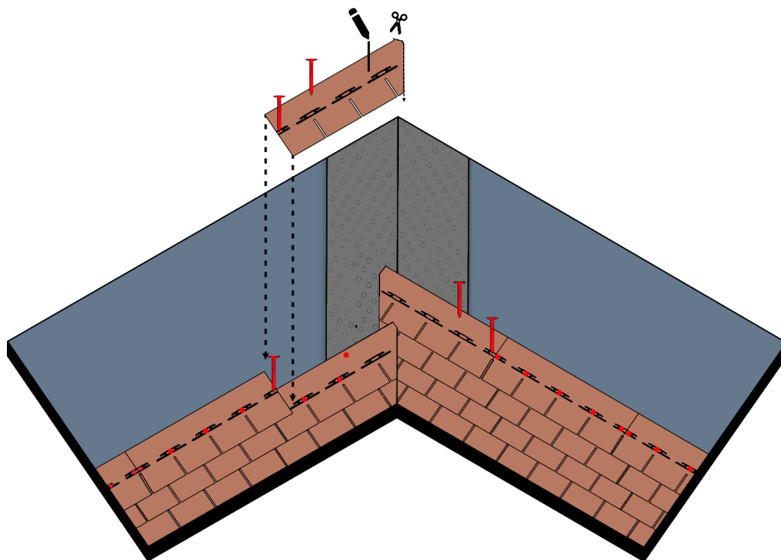
Fig. 14 - Shingles installation at valleys
