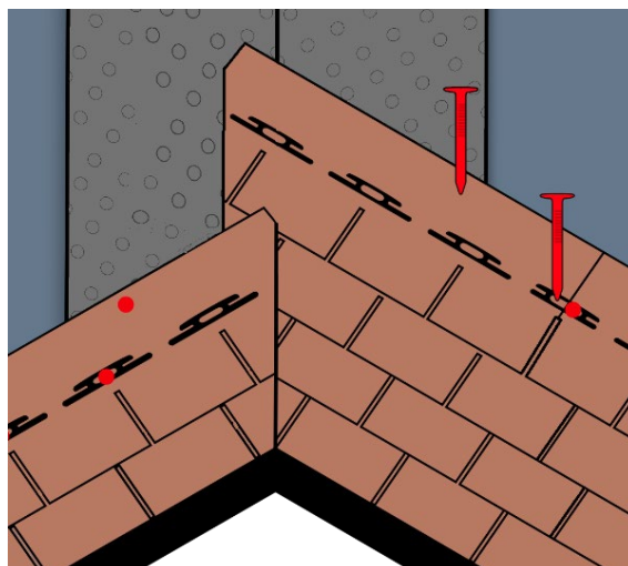
Fig. 13 - Shingles installation at valleys
