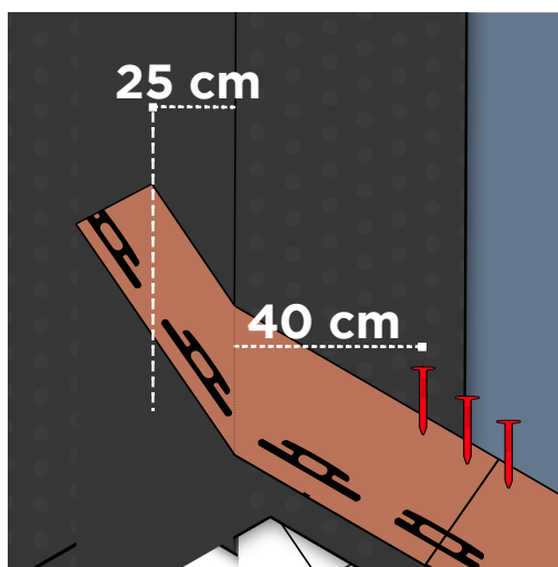
Fig. 12 - Shingles installation at valleys
