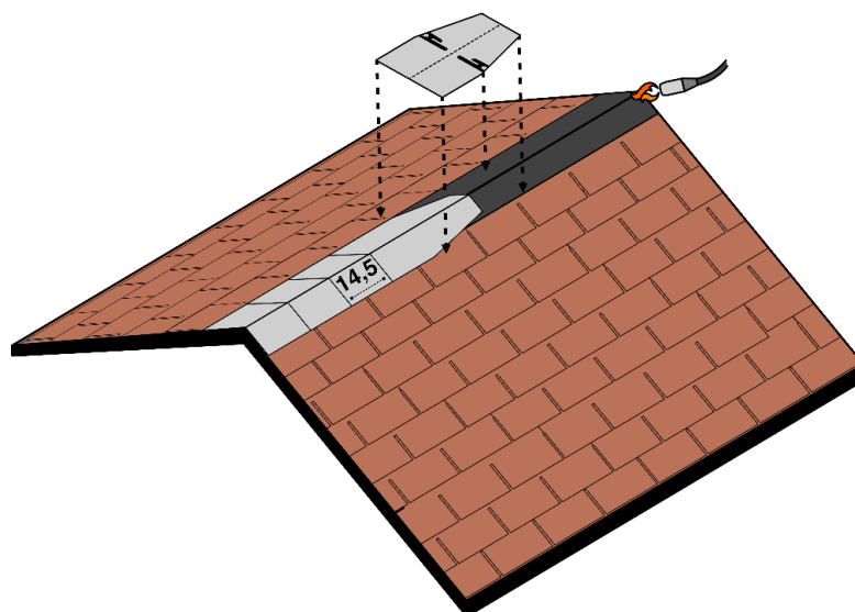
Fig. 19 – Ridge elements installation by torch
