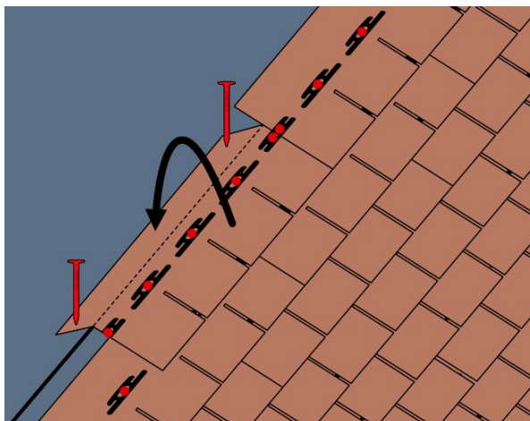
Fig. 9 - Shingles installation at the ridge
