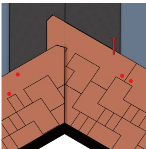
Fig. 13 - Shingles installation at valleys
